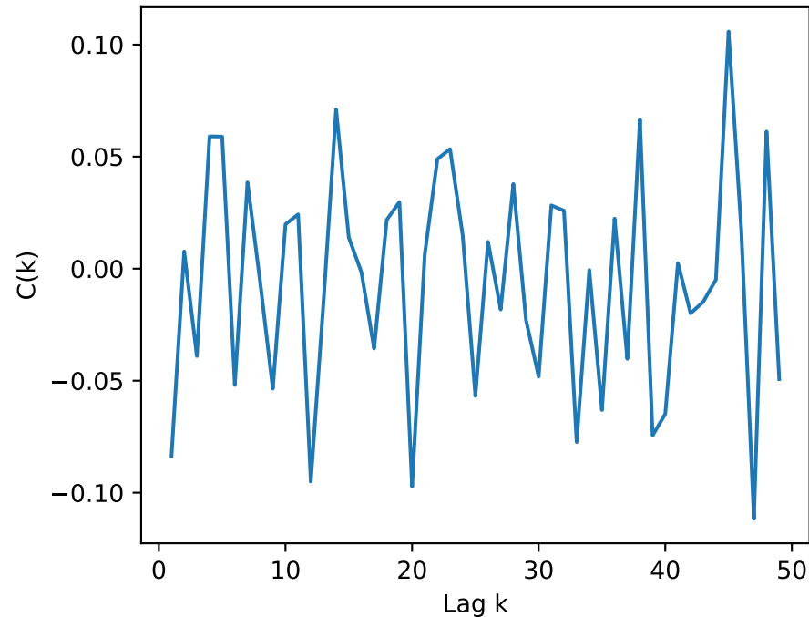
LUMO Autocorrelation
